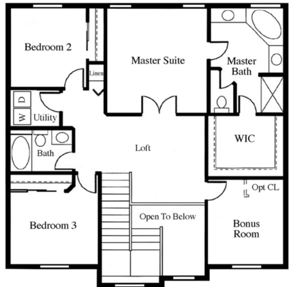
Second Floor
